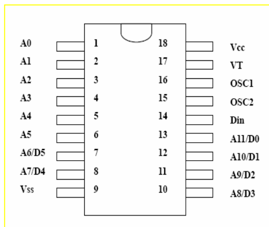
PT2272L4-DIP18
